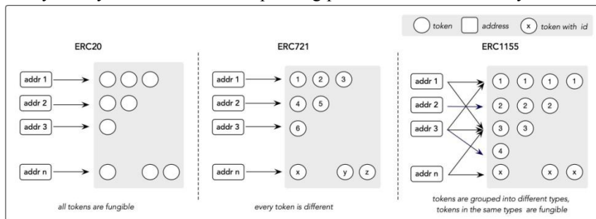
Fig.2: NFT-related Token Standard
