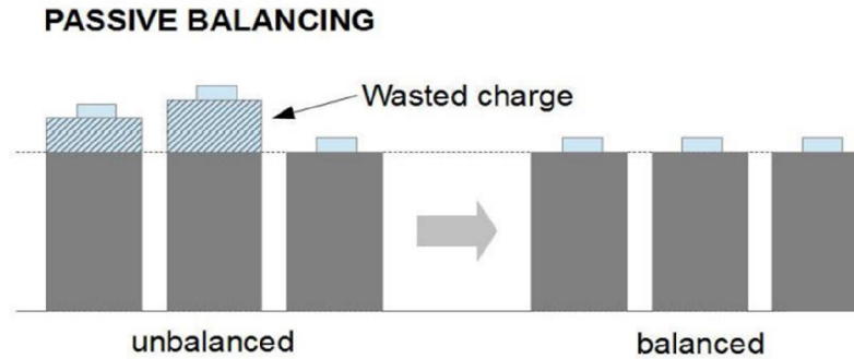
Figure 3: Passive Cell Balancing
