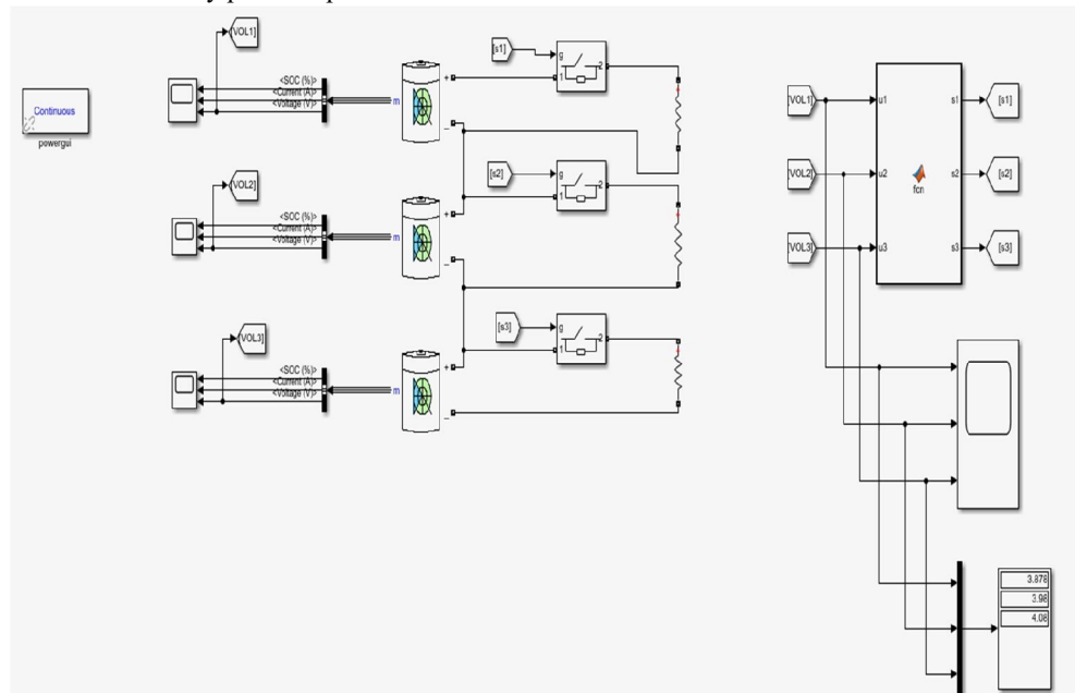
Figure 7: Simulation – Passive cell balancing
