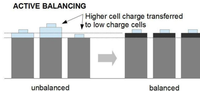
Figure 2: Active Cell Balancing
