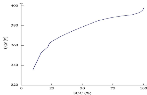
Figure 1: Relationship between SOC and OCV
