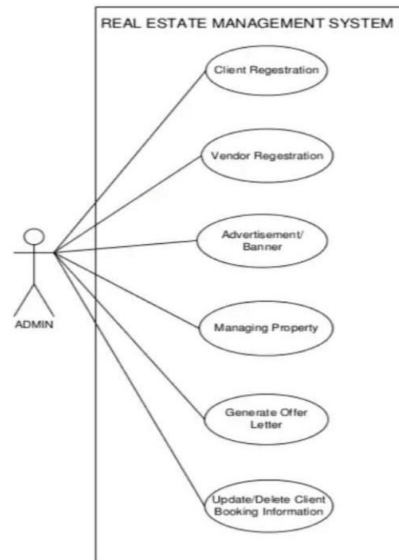
Fig 1: Admin Use Case Diagram
