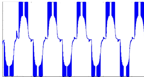
Figure 4: Output Voltage & Current of a Five Level DCMI.
