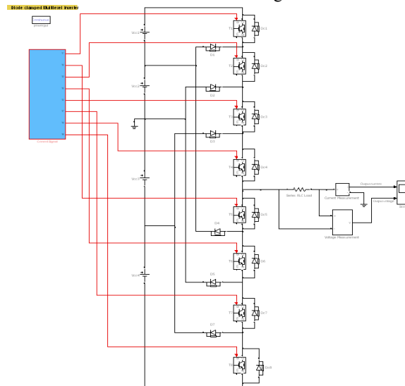
Figure3: Simulink Model of a Five Level DCMI. RESULTS:
