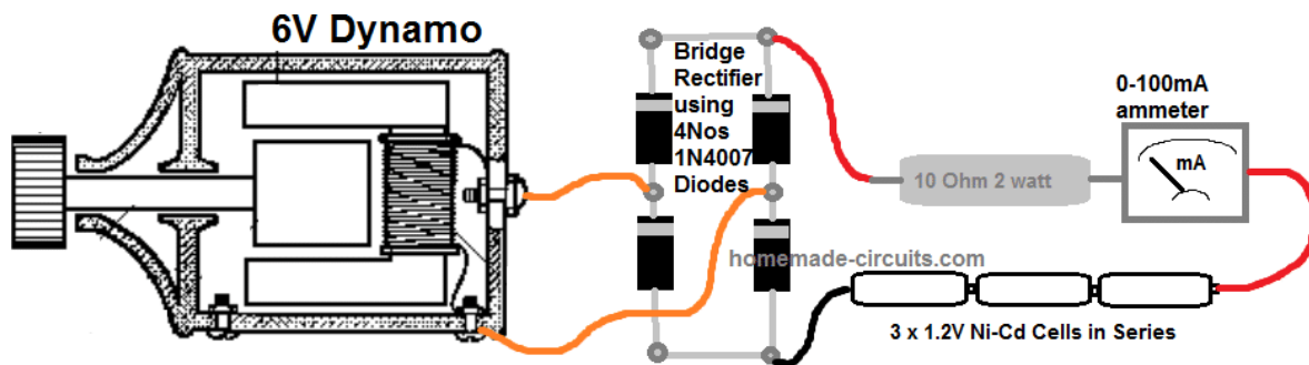
Fig. Block diagram of Dynamo
