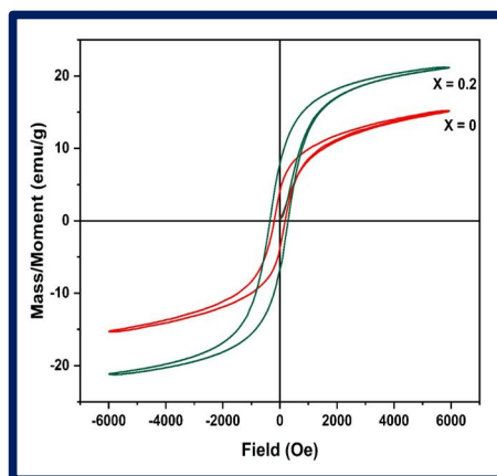
Fig 3: VSM of Mg 1-x Co x Fe 2 O 4 (x = 0, 0.2)
