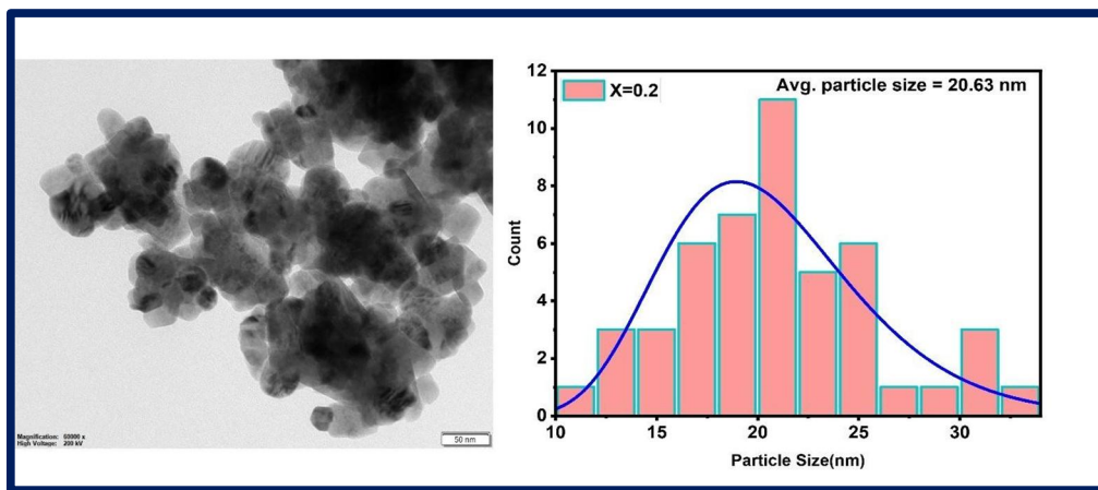
Fig 4: TEM of \text{Mg}_{1-x}\text{Co}_x\text{Fe}_2\text{O}_4 ( x = 0.2 )
