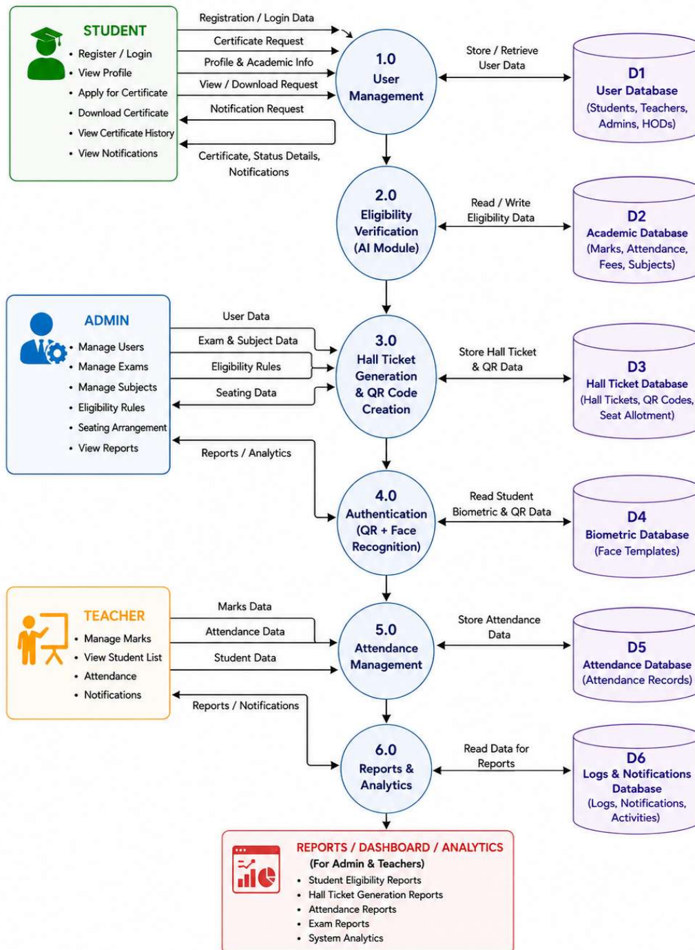
Figure 3: Workflow
