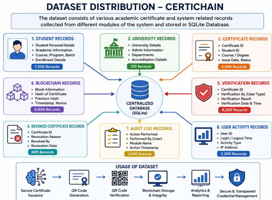
Figure 1: Dataset Distribution
