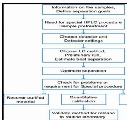
Figure2: Steps involved in HPLC Method development
