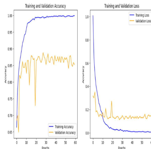
Figure 4: Accuracy and Loss Graph for DenseNet- MobileNet.
