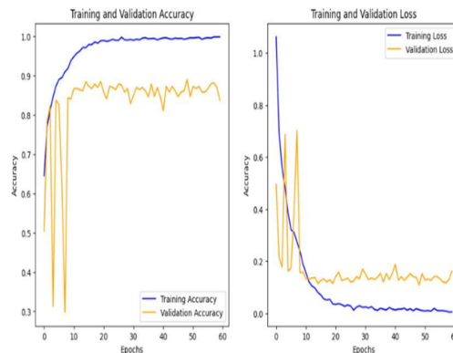
Figure 7: Accuracy and Loss Graph for DenseNet-AlexNet.
