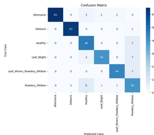
Figure 9: Confusion Matrix of DenseNet-ResNet50.
