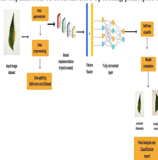
Figure 3: Functional Diagram of the Proposed Model.
