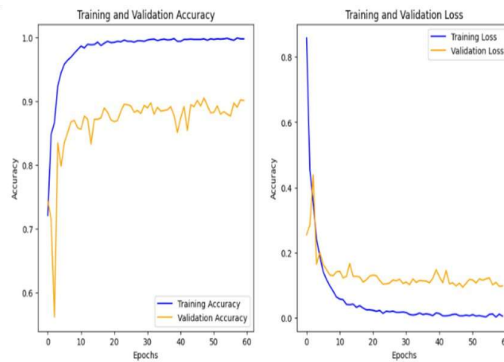
Figure 5: Accuracy and Loss Graph for DenseNet-ResNet5.
