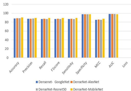
Figure 12: Comparison of used Models.
