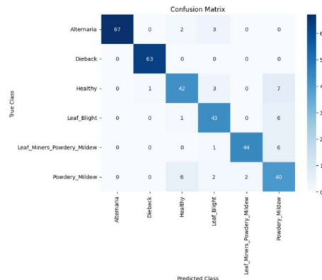
Figure 11: Confusion Matrix of DenseNet-AlexNet.
