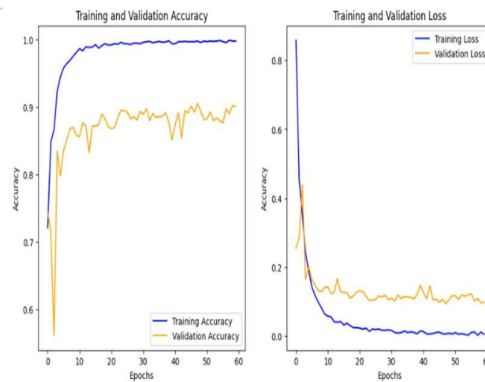
Figure 6: Accuracy and Loss Graph for DenseNet- GoogleNet.
