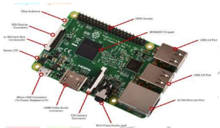
Fig 2: Raspberry Pi Module
