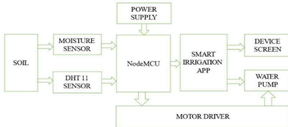
Fig. 1. Block Diagram of System
