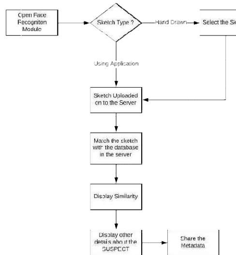
Fig. 8. Flow Chart for Recognizing a sketch in the application
