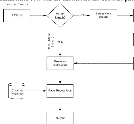
Fig. 6. System Flow of the application
