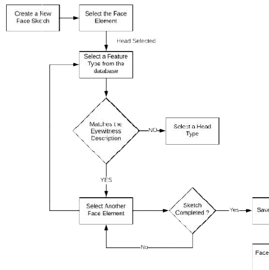
Fig. 7. Flow Chart for Creating a sketch in the application
