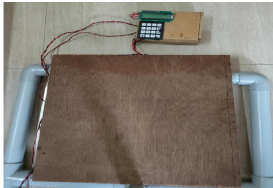
(Fig-5.3- The base for Weight Measurement)
