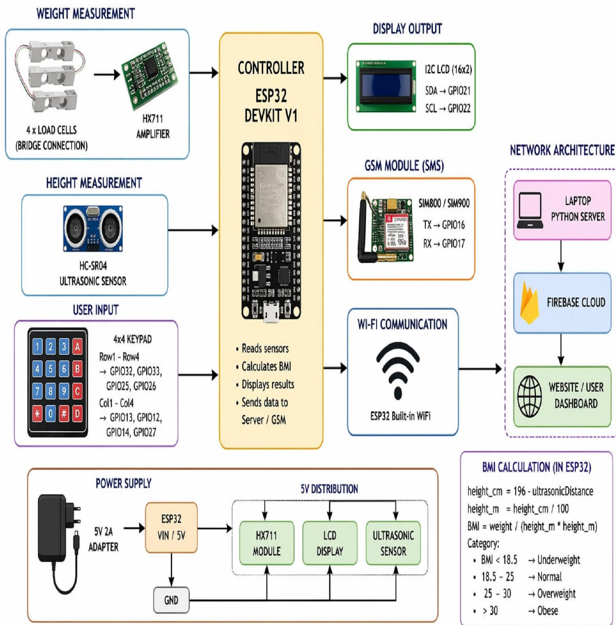
(Fig-3.1 Block Diagram of BMI System)
