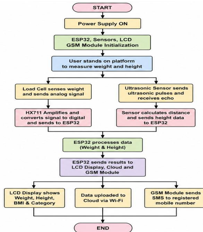
(Fig-3.3 Hardware Flowchart)
