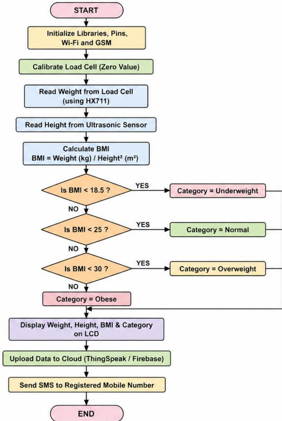
(Fig-3.2 Software Flowchart)
