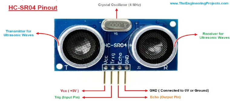
(Fig. 4.4 – Ultrasonic Sensor)
