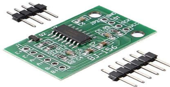
(Fig. 4.3 – HX711 Amplifier Module)
