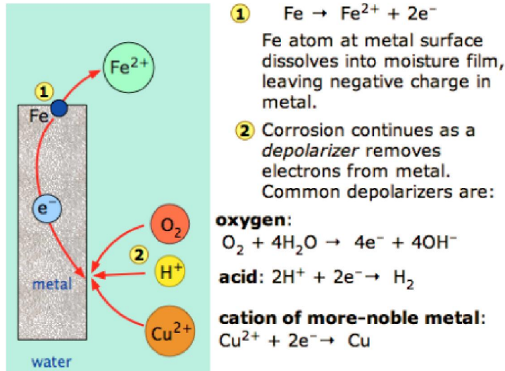
Fig.1 Mechanism of Corrosion
