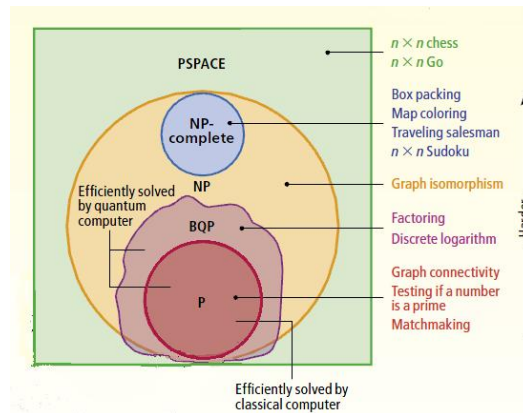
Fig 2: Various classes of computational problems
