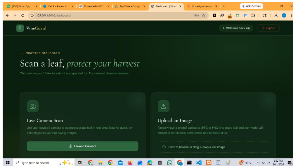
Fig 3. Dashboard
