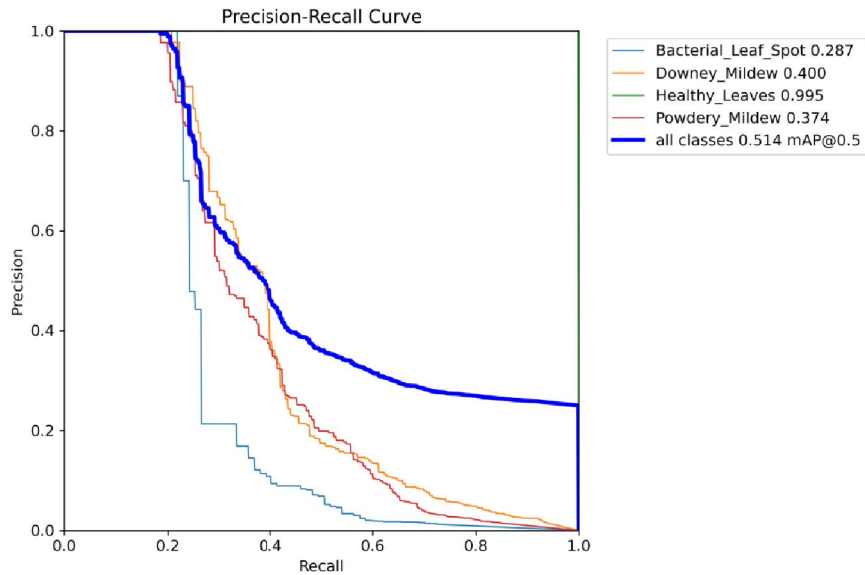
Fig 5. Precision-Recall
