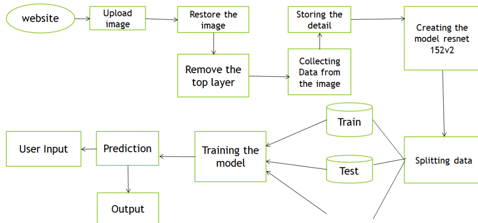
Fig 1.Architecture
