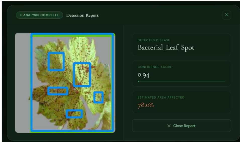
Fig 4. Detection Module
