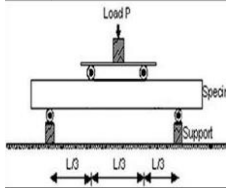
FIG 2. LOADING SETUP
