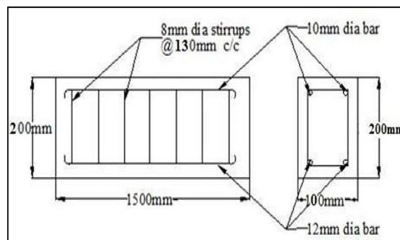
FIG I. RCC BEAM
