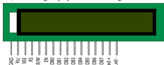
Figure 6: LCD display
