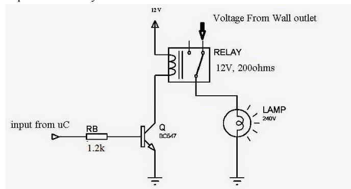
Figure 5: Relay Driver Circuit
