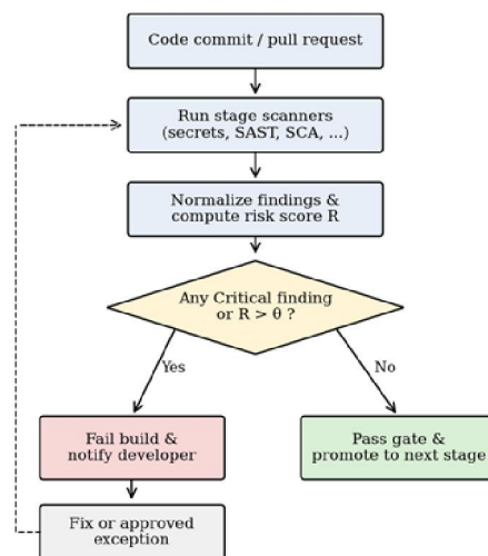
Fig. 2. Security gate decision flow applied at each stage.
