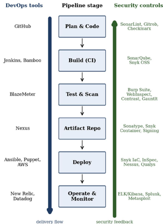
Fig. 1. Proposed DevSecOps toolchain framework with DevOps tools and security controls mapped to each CI/CD stage.
