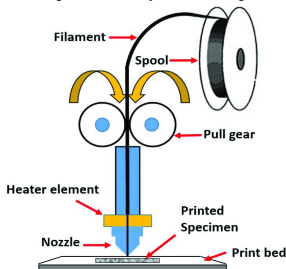
Figure 4 - Fused Deposition Modeling.
