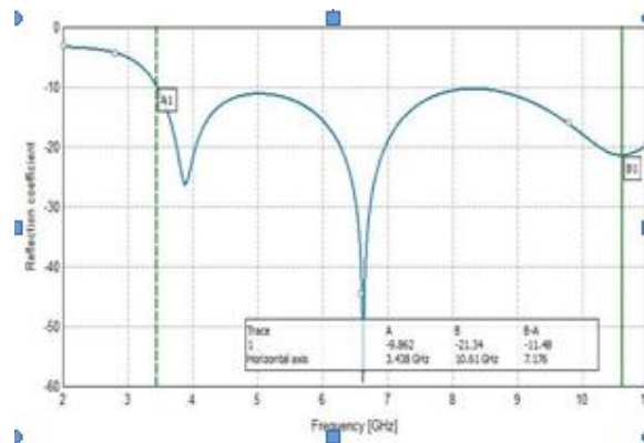
Figure 2. Reflection coefficient magnitude of proposed antenna.
