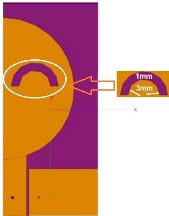
Figure 1. Proposed antenna geometrical details.
