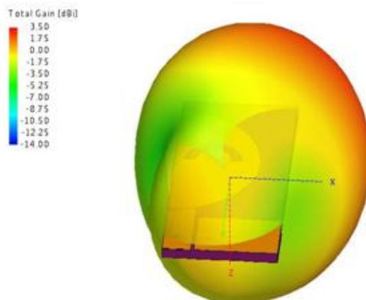
Figure 8. 3D gain of proposed antenna.
