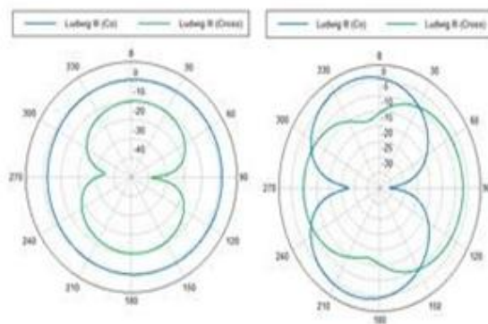
Figure 6. Radiation Patterns of proposed antenna.
