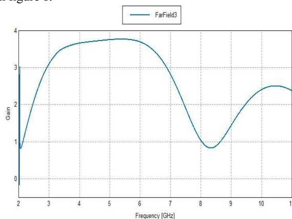
Figure 7. Gain of proposed antenna.
