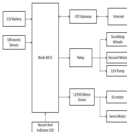
Figure 2: Block Diagram
