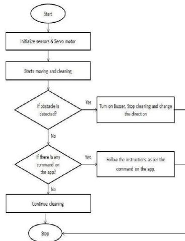
Figure 3: Flowchart
