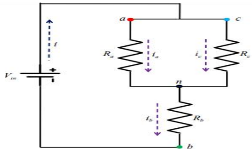
Figure 3.5: Equivalent circuit in Mode 1
