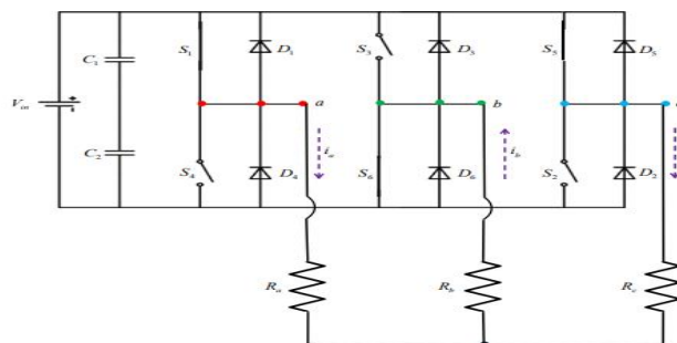
Figure 3.4: Current through the load in Mode 1
