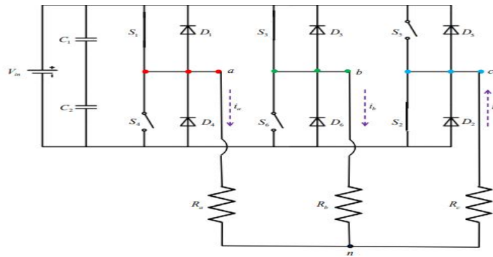
Figure 3.8: Current through the load in Mode 3
