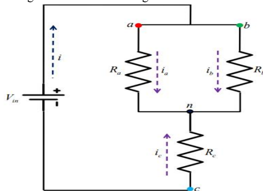
Figure 3.9: Equivalent circuit in Mode 3
