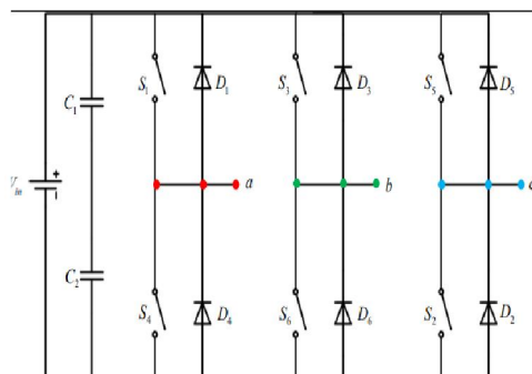
Figure 3.2: Three phase inverter configuration
