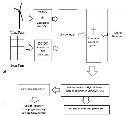
Figure 1: Block diagram of proposed Hybrid power system
