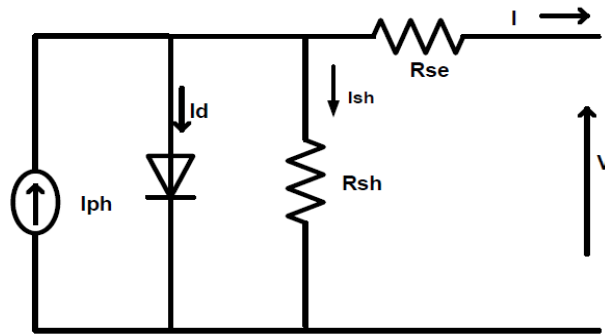
Fig. 3.15 Equivalent circuit of single diode solar cell
