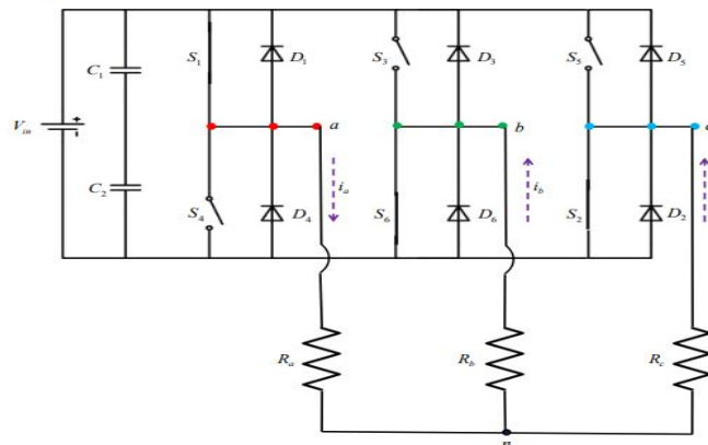
Figure 3.6: Current through the load in Mode 2
