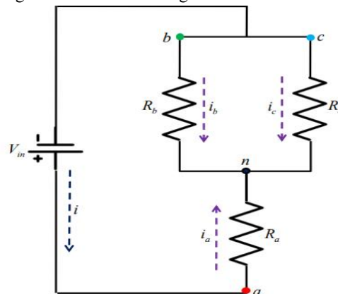
Figure 3.7: Equivalent circuit in Mode 2
