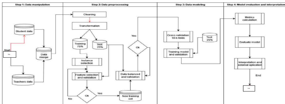
Fig1.WorkFlow of System
