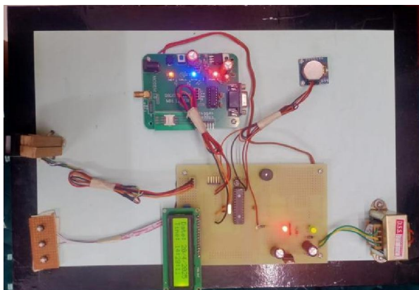
Figure 7. Actual Portable fingerprint Attendance System
