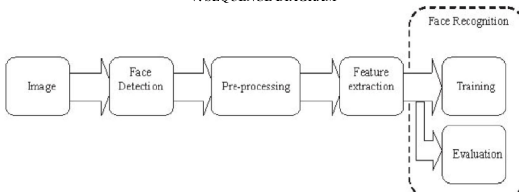
Fig 5.1 sequence diagram
