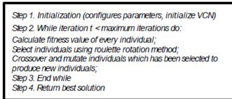
Fig 2 Genetic Algorithm
