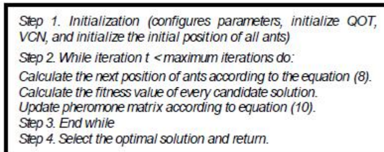
Fig 3 ACO Algorithm
