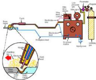
Fig. 3 Gas Metal Arc Welding M/C
