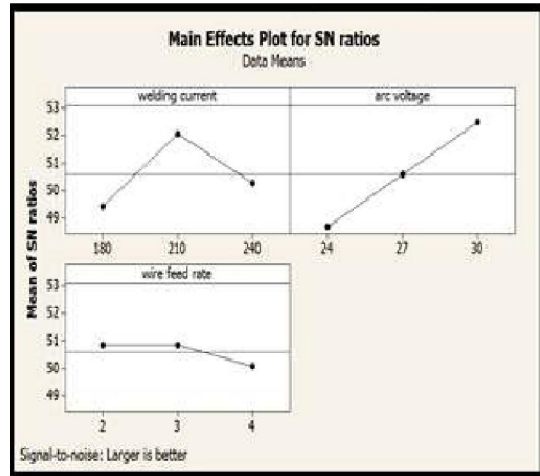
Fig.7 Main effect plot for SN ratios
