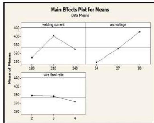
Fig.6 Main effect plot for means
