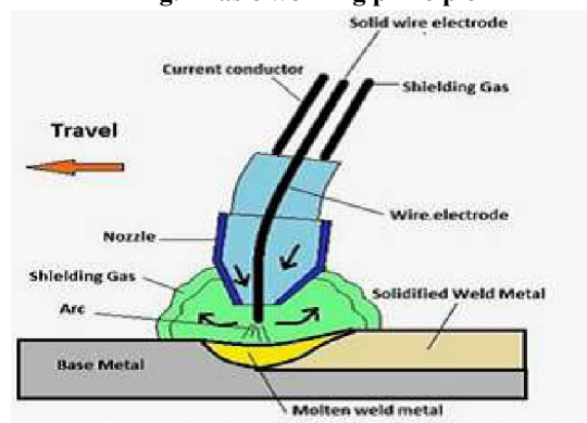
Fig.2 Schematic of GMAW
