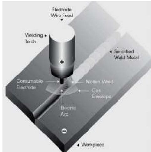
Fig.1 Basic working principle
