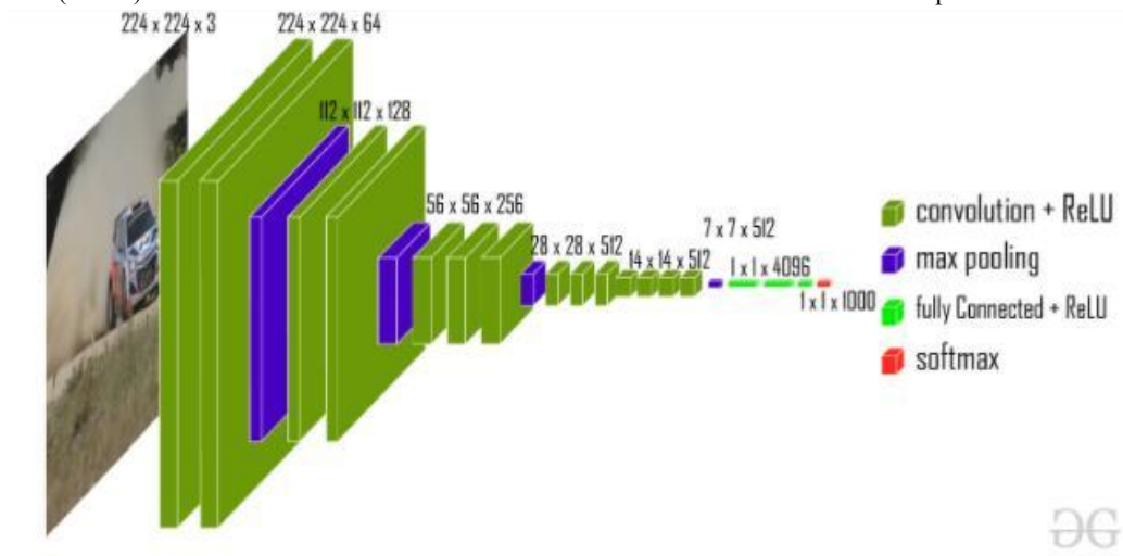
Figure 1: VGG 32 Model
