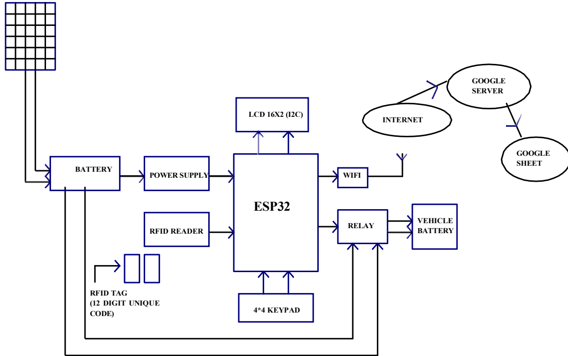
Figure 1: Block Diagram
