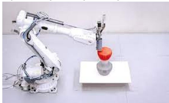
Fig. 5: Robotic Arm & Hybrid FDM 3D printing
